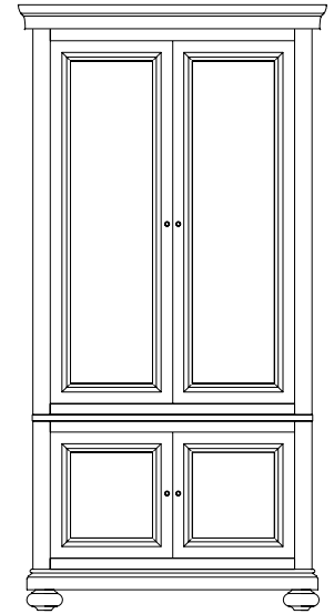
GLASS DISPLAY CABINET H: 1913 W: 938 D: 400
