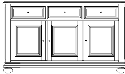
LARGE SIDEBOARD WITH 3 DOORS 3 DRAWERS H: 868 W: 1500 D: 470
