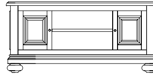
STANDARD TV CABINET H: 520 W: 1100 D: 470
