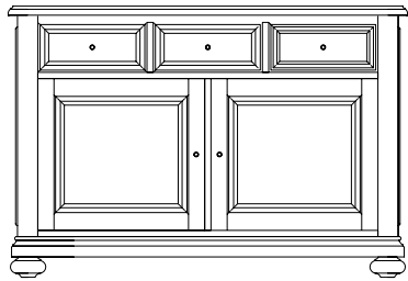
SMALL SIDEBOARD WITH 2 DOORS 3 DRAWERS H: 868 W: 1280 D: 470
