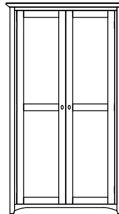
FULL LENGTH WARDROBE H: 1910 W: 1095 D: 580
