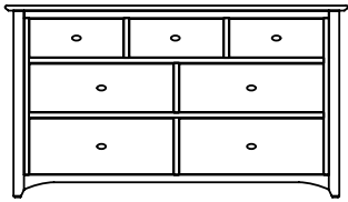
3 OVER 4 CHEST H: 770 W: 1375 D: 420
