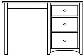
SINGLE DRESSING TABLE H: 770 W: 1195 D: 420
