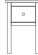
LAMP TABLE WITH DRAWER H: 560 W: 400 D: 400
