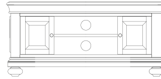
STANDARD TV CABINET H: 518 W: 1110 D: 460
